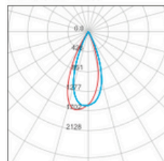
Narrow 38° 10W
